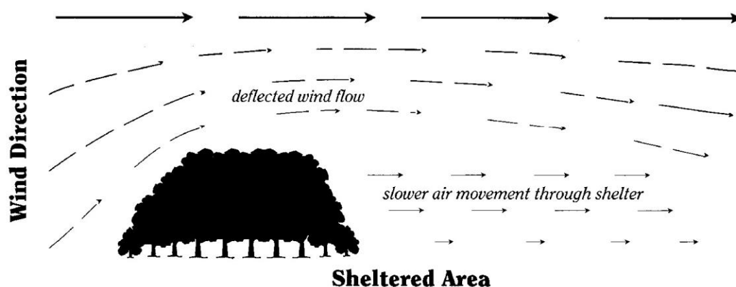
Figure 2: Illustration of wind flow and shelter created by a shelterbelt (J. Davis).
